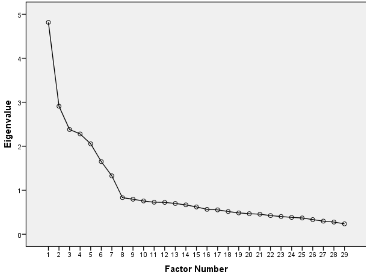
Scree Plot
